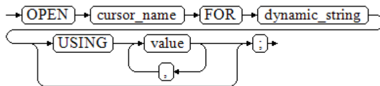
图 12-9 open_for::=
