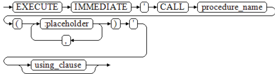
图 12-12 call_procedure::=
